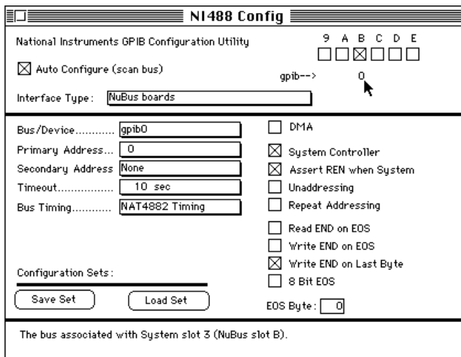
Figure 3-3. Sample Configuration for the GPIB Board
